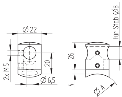
Abb. Variante Links
